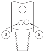
CGA 910 Pin-Indexed Yoke, Pins 3-5
