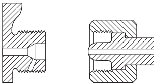
CGA 326 .825-14NGO-RH-EXT (Small Round Nipple)
