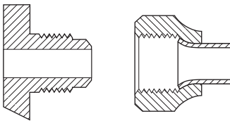
CGA 295 .750-16UNF-2A-RH-EXT (1/2" SAE Flare)
