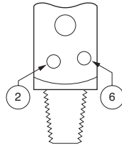
CGA 880 Pin-Indexed Yoke, Pins 2-6
