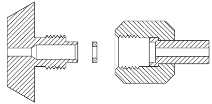
CGA 280 .745-14NGO-RH-EXT
