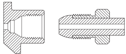
CGA 296 .803-14UNS-2B-RH-INT
