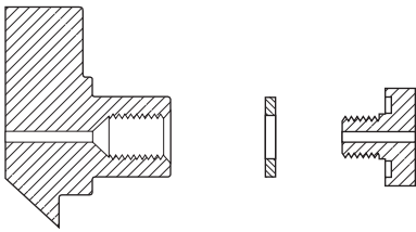
CGA 110 .3125-32UNEF-2B-RH-INT
