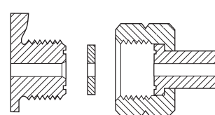
CGA 330 .825-14NGO-LH-EXT (Flat Nipple)
