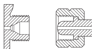
CGA 350 .825-14NGO-LH-EXT (Round Nipple)
