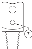
CGA 965 Pin-Indexed Yoke, Pin No. 7
