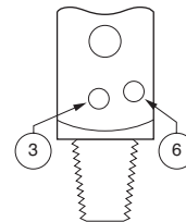
CGA 920 Pin-Indexed Yoke, Pins 3-6
