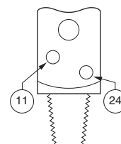
CGA 973 Pin-Indexed Yoke, Pins 11-24
