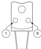
CGA 940 Pin-Indexed Yoke, Pins 1-6
