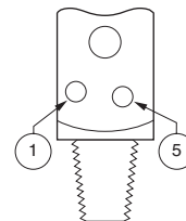
CGA 950 Pin-Indexed Yoke, Pins 1-5
