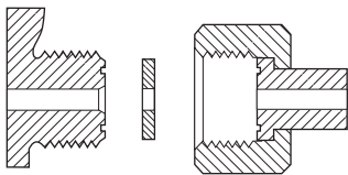
CGA 320 .825-14NGO-RH-EXT (Flat Nipple)
