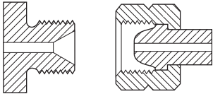
CGA 290 .745-14NGO-LH-EXT
