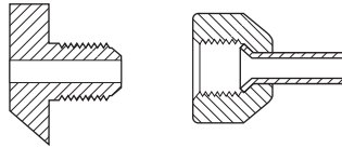
CGA 240 .375-18NGT-RH-INT
