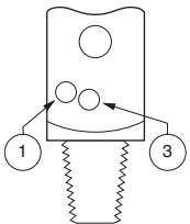
CGA 900 Pin-Indexed Yoke, Pins 1-3
