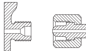
CGA 280 .745-14NGO-RH-EXT
