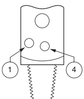
CGA 960 Pin-Indexed Yoke, Pins 1-4
