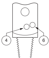
CGA 930 Pin-Indexed Yoke, Pins 4-6
