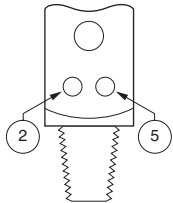
CGA 870 Pin-Indexed Yoke, Pins 2-5
